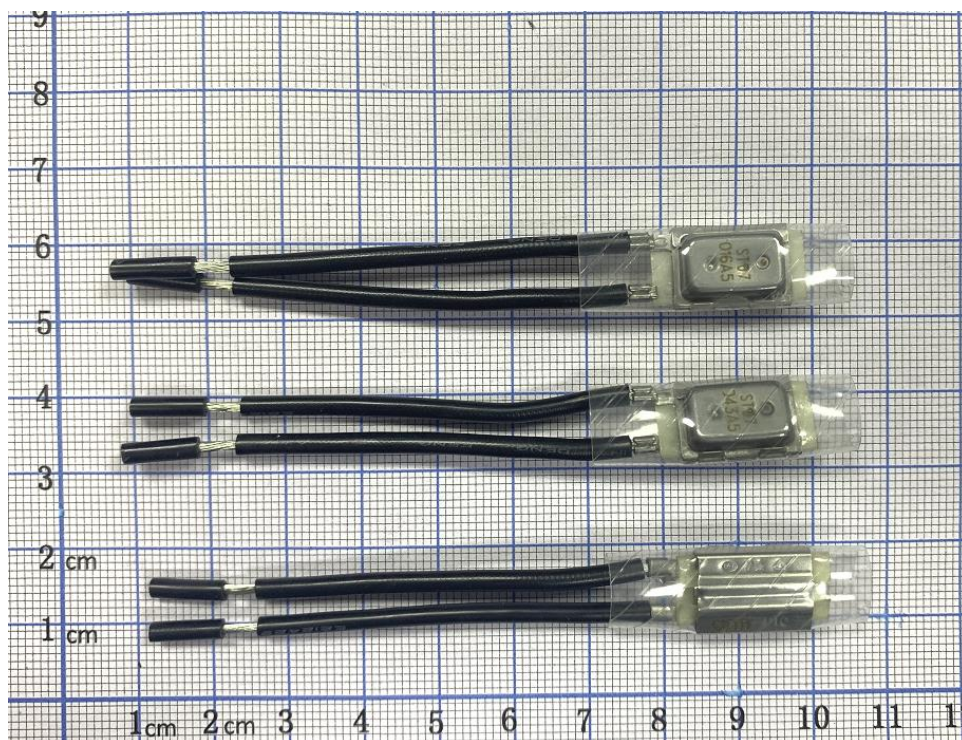
Appearance of Model ST07016A5PTC, ST07043A5PTC
