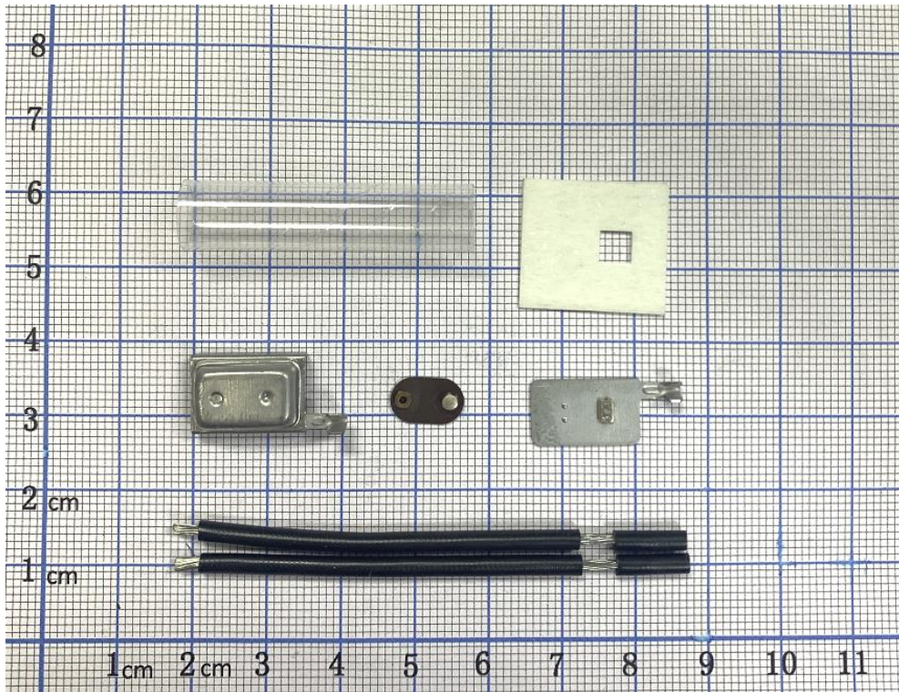
Model ST07016A5, ST07043A5 internal structure diagram
